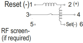
Circuit Diagram, Latching
